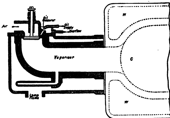
FIG. 29.—Crossley Vaporizer.
